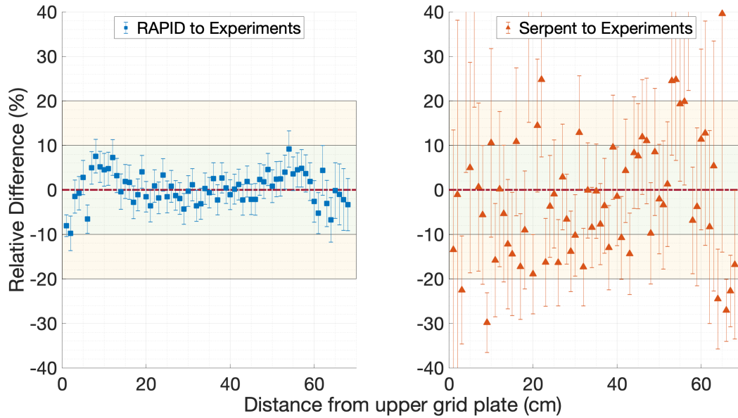
^{197}\text{Au}(n, \gamma) reaction rates relative differences - July 23, 2012 - MP16
