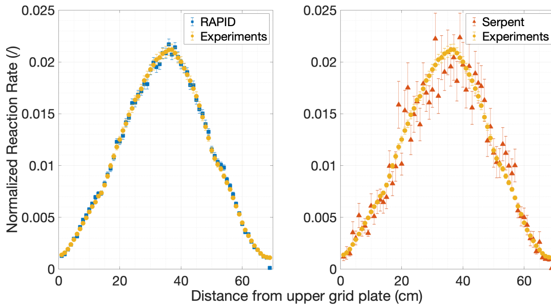
^{197}\text{Au}(n, \gamma) reaction rates comparison - July 23, 2012 - MP16
